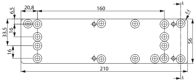
Replacement plate A124 For renovation applications
