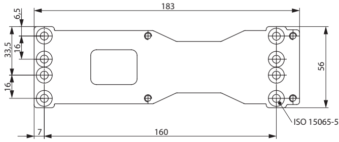
Mounting plate A120 For mounting with drilling template acc. to EN 1154 Supplement 1 and for universal use
